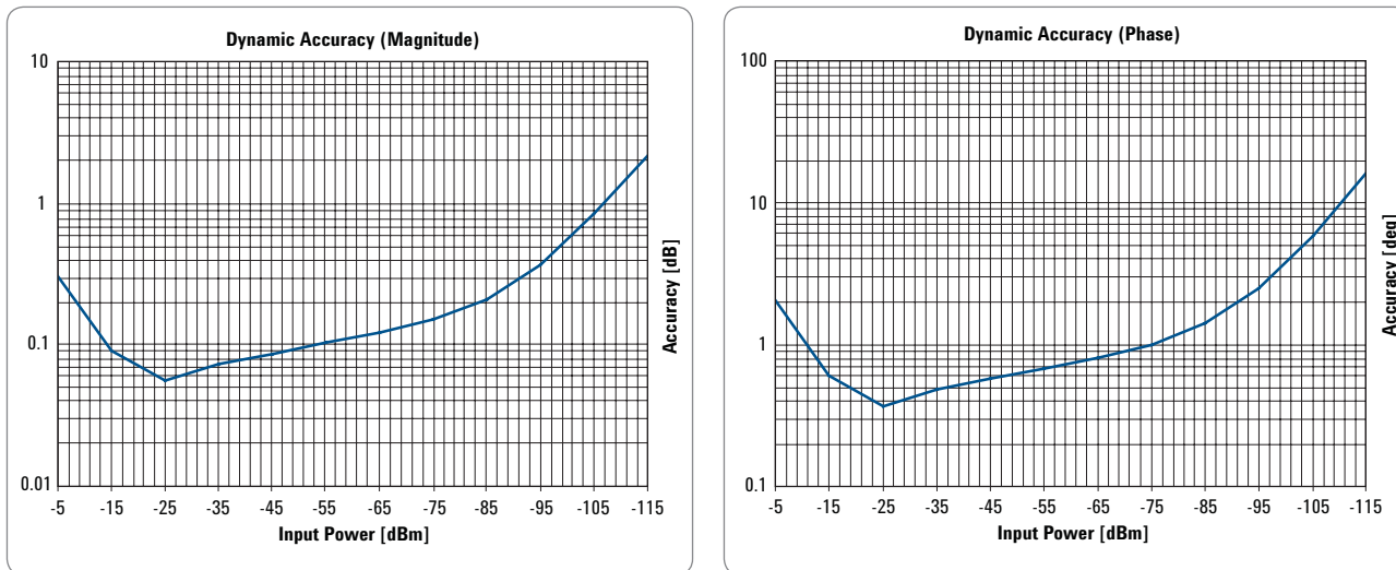
Figure 20. Dynamic Accuracy
