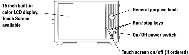
Figure 8. 16800 Series front panel
