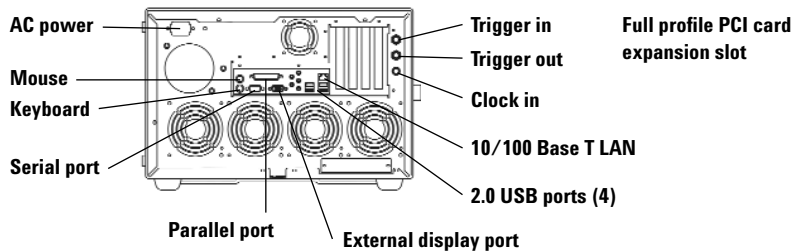
Figure 9. 16800 Series back panel
