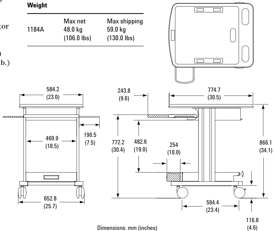
Figure 12. Agilent 1184A testmobile cart dimensions
