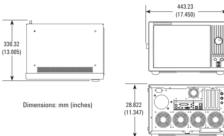
Figure 7. 16800 Series exterior dimensions.
