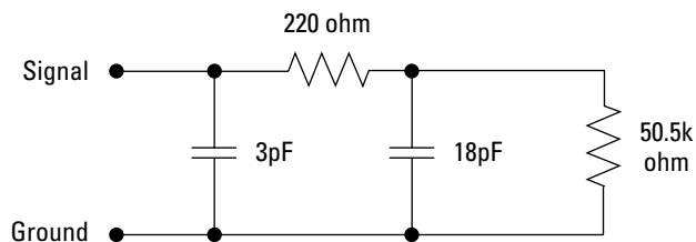
Figure 6.8. E5339A equivalent load.
