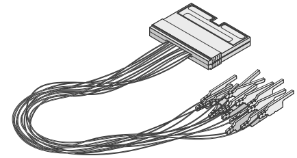
NEW Figure 3.3. The E5381A (differential) and E5382A (single-ended) flying lead probe sets provide connections for 17 channels of the 16753A, 16754A, 16755A, 16756A and 16760A logic analyzers.
