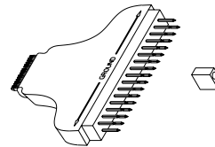
Figure 3.6. Wedge adapters connect to multiple pins of 0.5 mm or 0.65 mm QFP ICs. Refer to "Probing Solutions for Agilent Technologies Logic Analysis Systems," publication number 5968-4632E, for specific part numbers.
