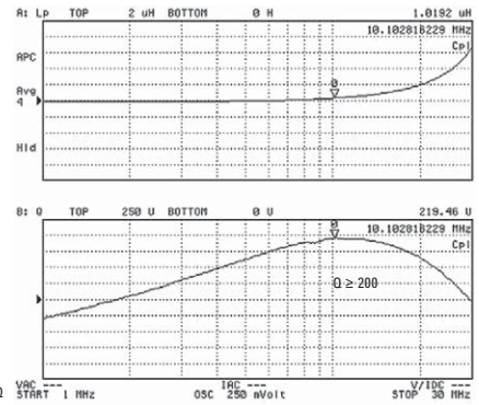
High Q inductor measurement (low-loss)
