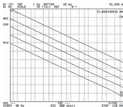
SMD capacitor impedance measurement (using the 42942A)
