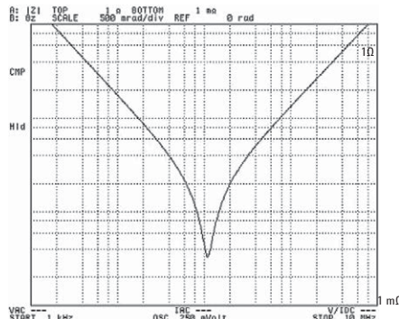
Low-loss capacitor ESR (equivalent series resistance) measurement (100 \mu F ceramic C)
