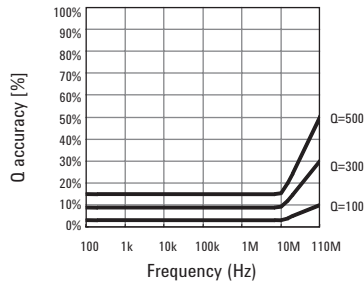
4294A Q accuracy (typical) OSC level = 250 mV
