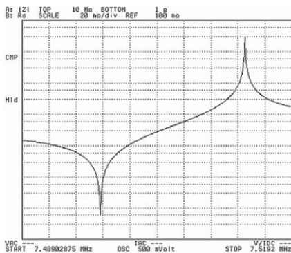
Crystal resonator impedance measurement
