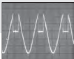
Sine wave with the positive halfcycle clipped at 0V from 50° - 130°
